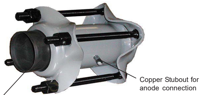
Insulating Sleeve
